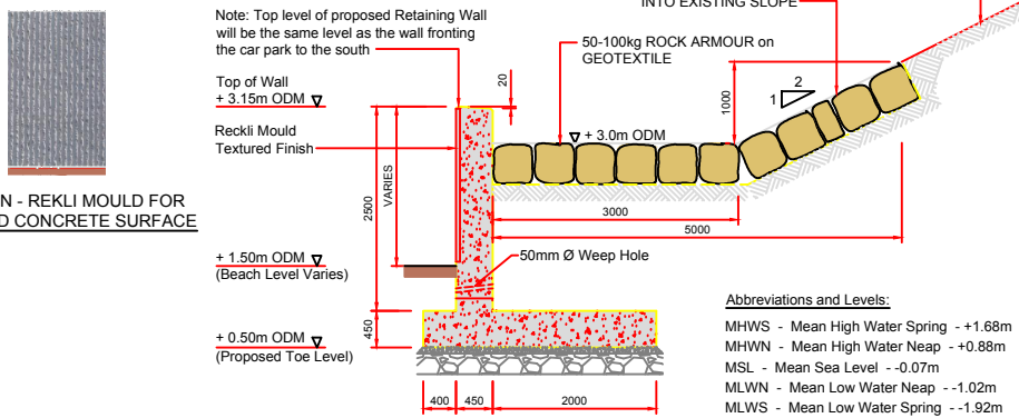
RETAINING WALL SECTION Scale 1:50
