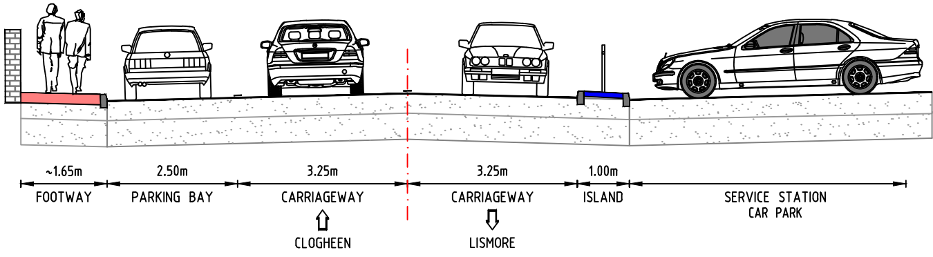
CROSS SECTION 1-1 R668 Proposed Cross Section
