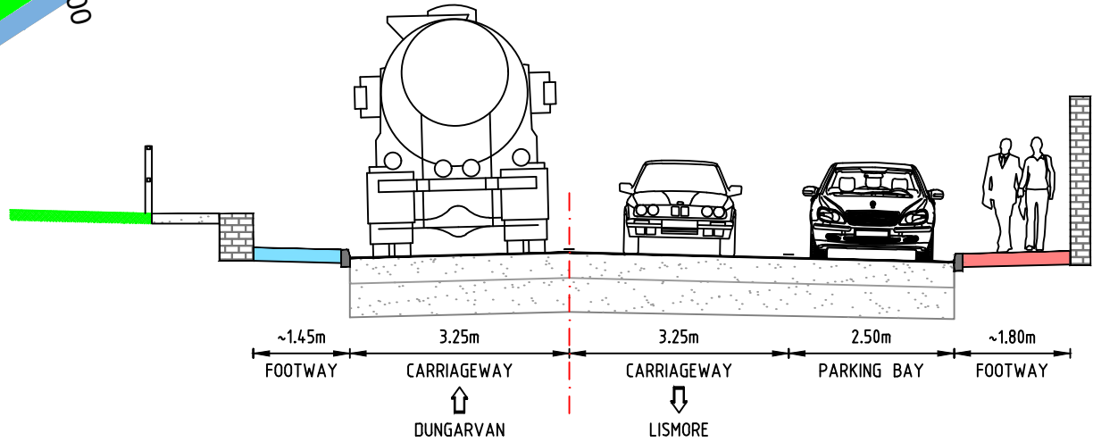
CROSS SECTION 2-2 N72 Proposed Cross Section
