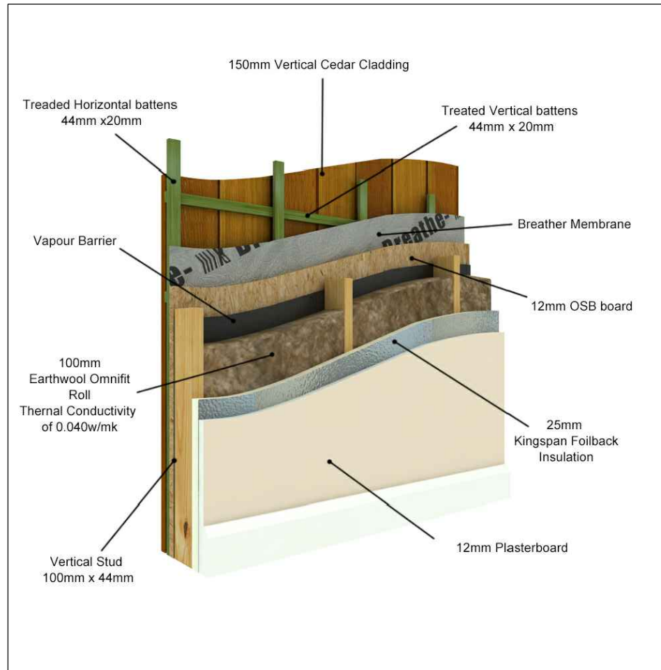
7 02 WALL DETAIL NTS
