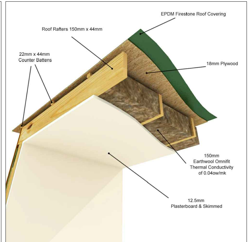
7 03 ROOF DETAIL NTS
