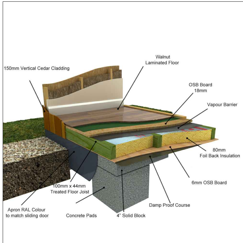
7 01 FLOOR DETAIL NTS
