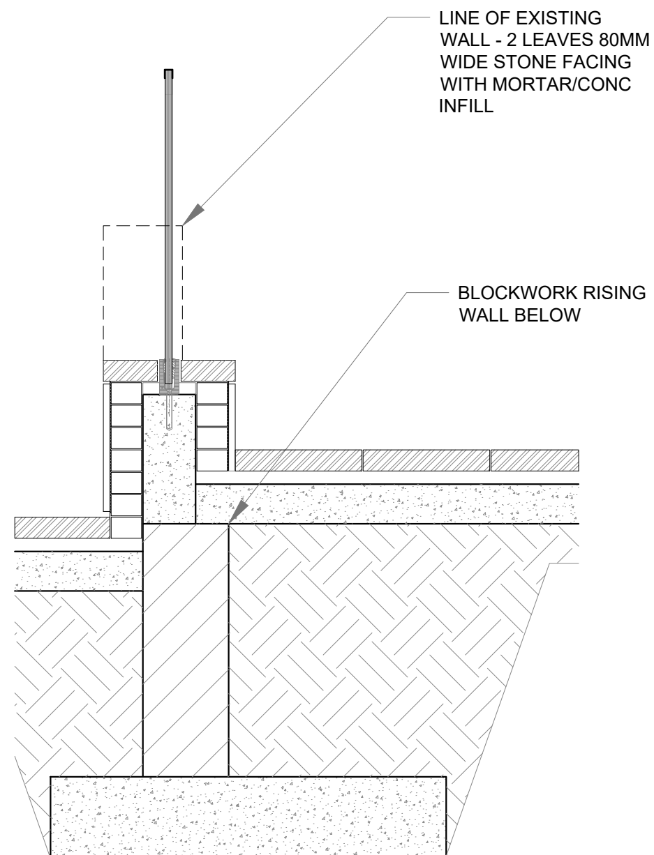
S5 01 NEW GLASS BALUSTRADA RETURN DERTAIL SCALE: 1:20 @ A3
