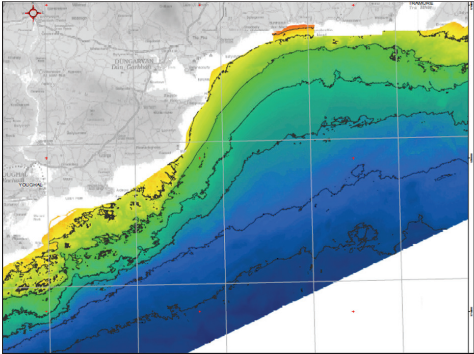
Figure 8.3 Seabed depths off the Coast of Waterford [Source: INFOMAR]
