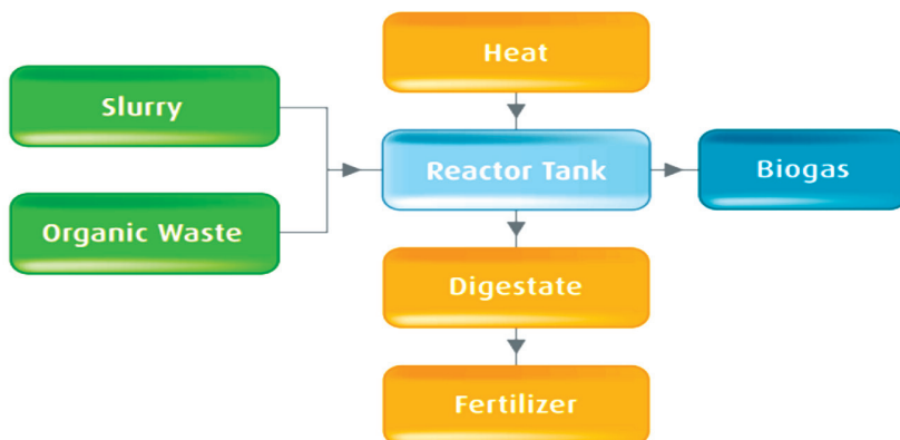
Figure 7.2 Anaerobic Digestion Diagram [Source: South-East Bio-Energy Implementation Plan 2013-2020]
