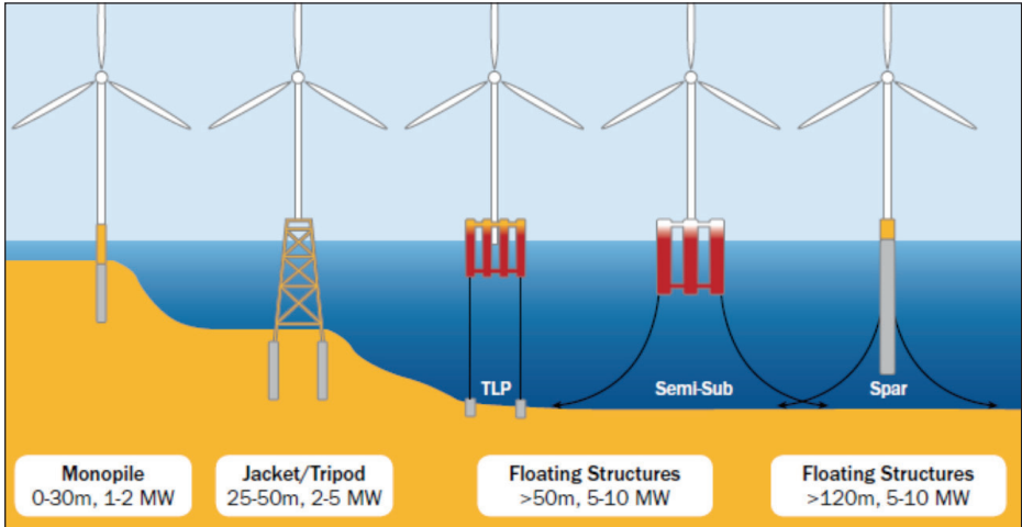
Figure 8.2 Offshore wind foundations [Source: European Wind Energy Association 2013]
