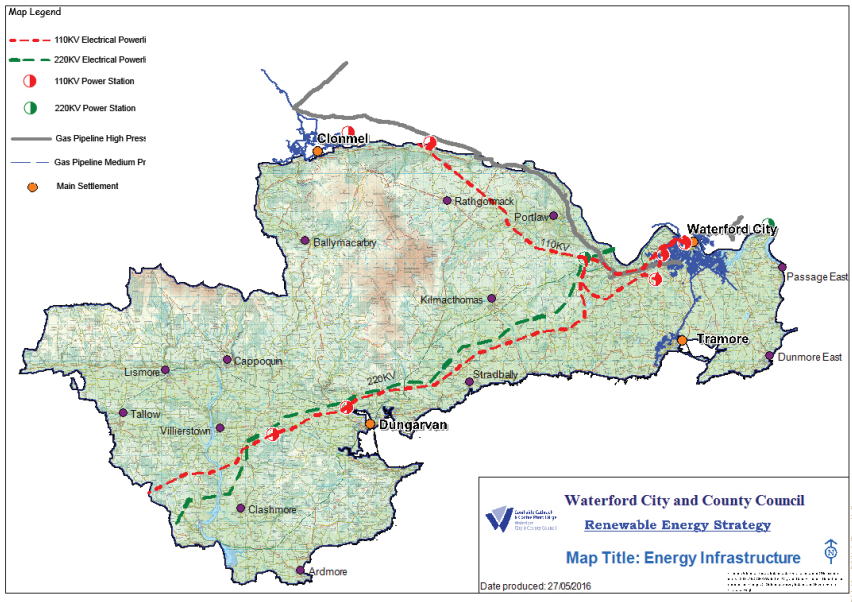
Figure 12.1 Energy Infrastructure in Waterford
