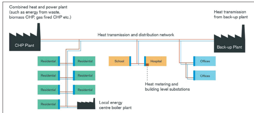
Figure 7.3 District Heating scheme example. (source: www.londonheatmap.org.uk )
