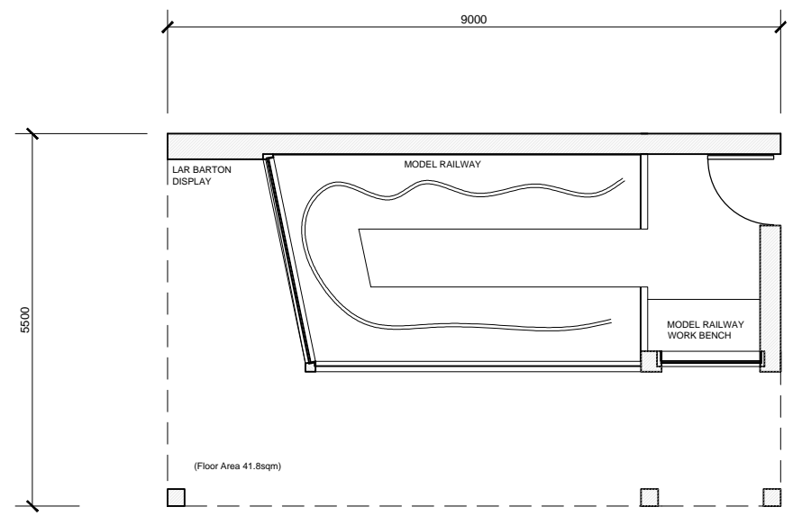
Proposed Rail Model Floor Plan, scale 1:100
