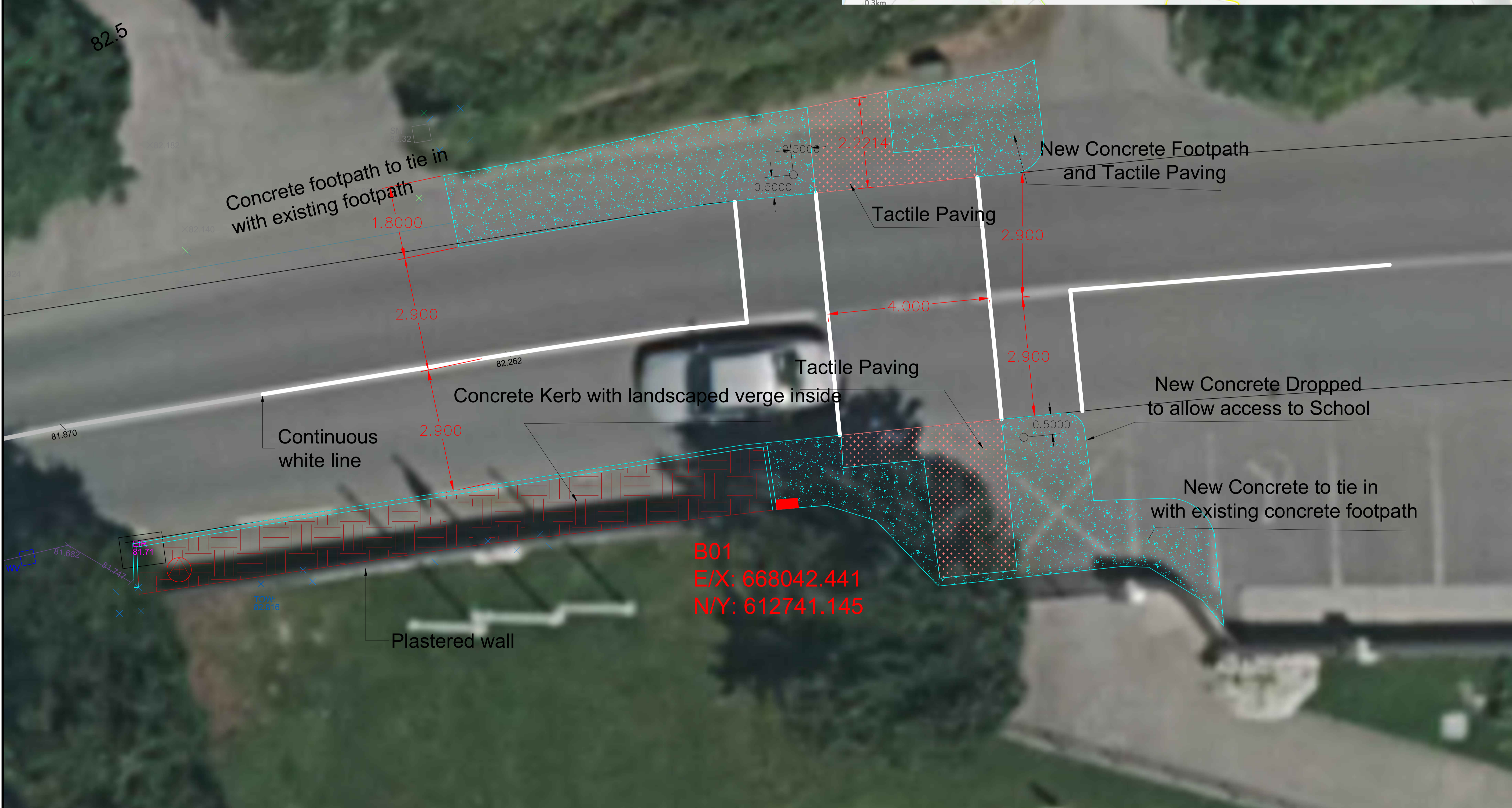
Figure 7.53: Signalised Pedestrian Crossing
