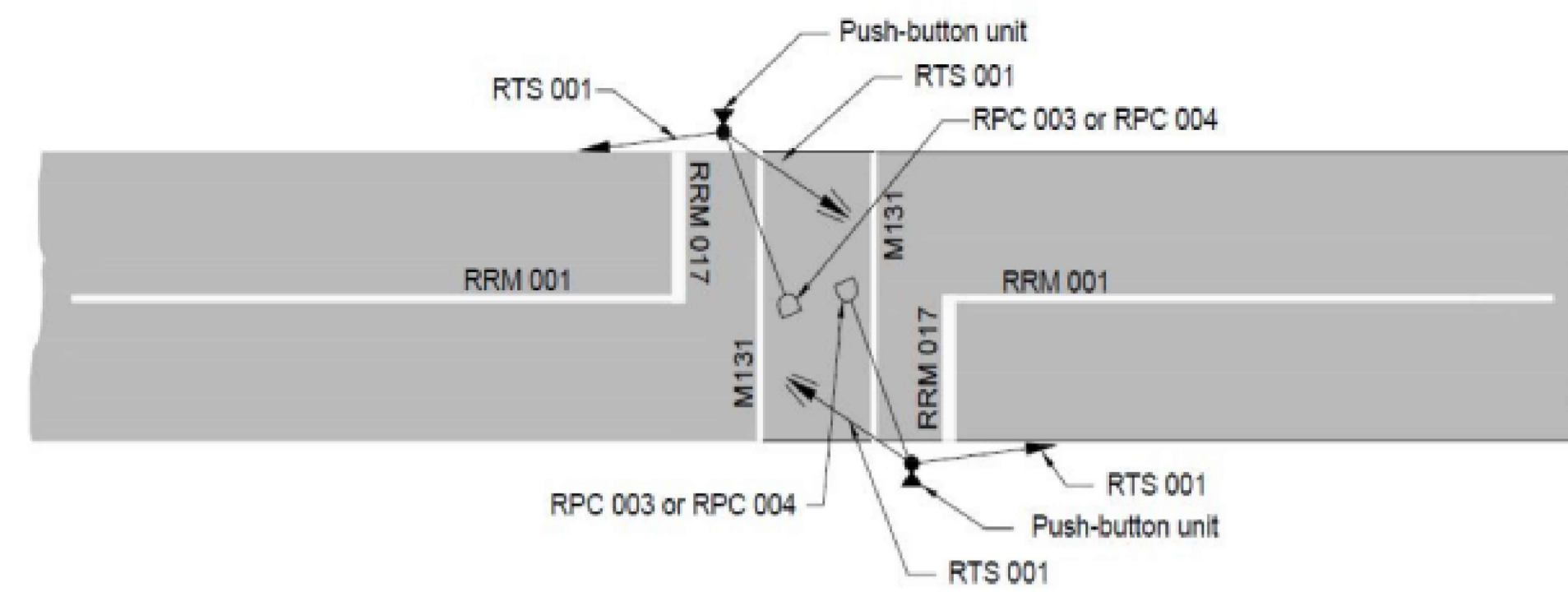
Figure 7.53: Signalised Pedestrian Crossing
