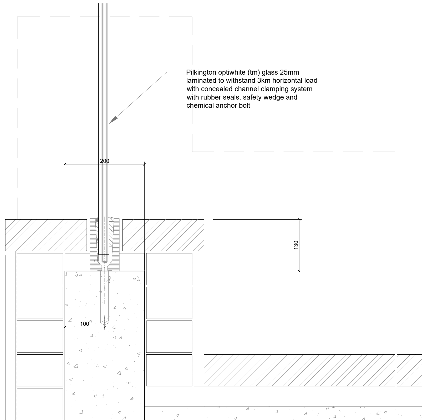
S6 01 DETAIL OF GLASS BALUSTRADE SCALE: 1:5 @ A3
