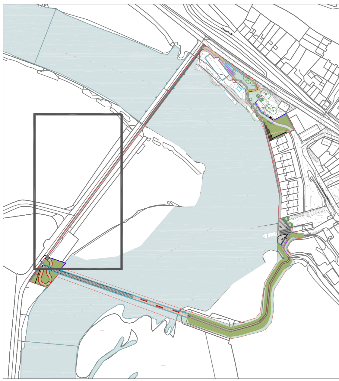
LOCATION PLAN (ROUTE-WIDE) 1:2500
