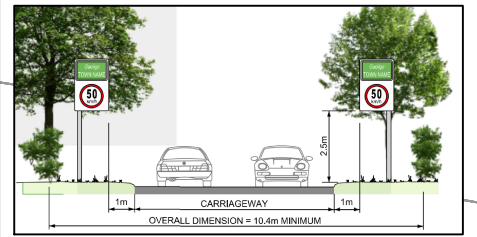
DETAIL FOR TII GATEWAY: TYPE A DESIGN
