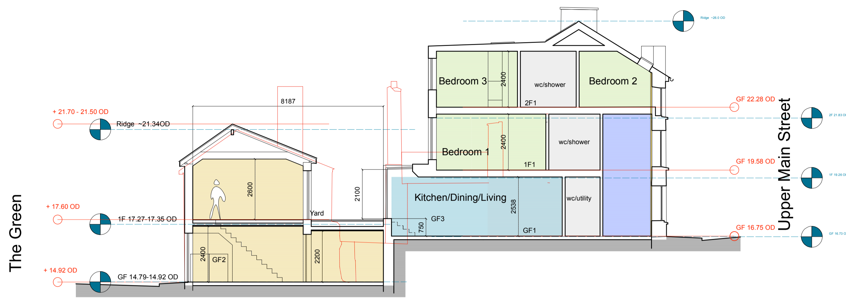
Section B-B (Typical Section House 7 and 8 - Proposed)
