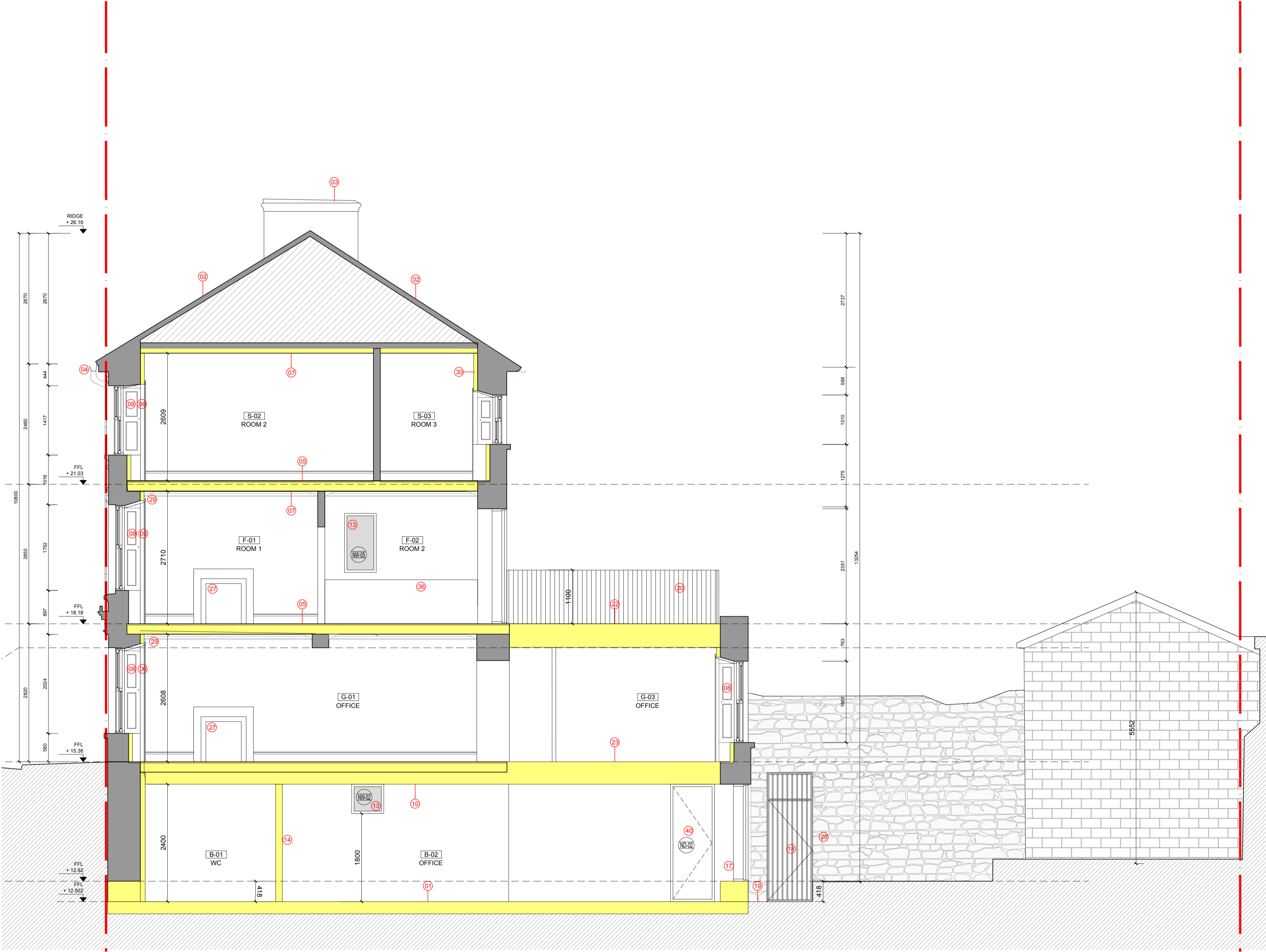
01 PROPOSED SECTION AA 1:50
