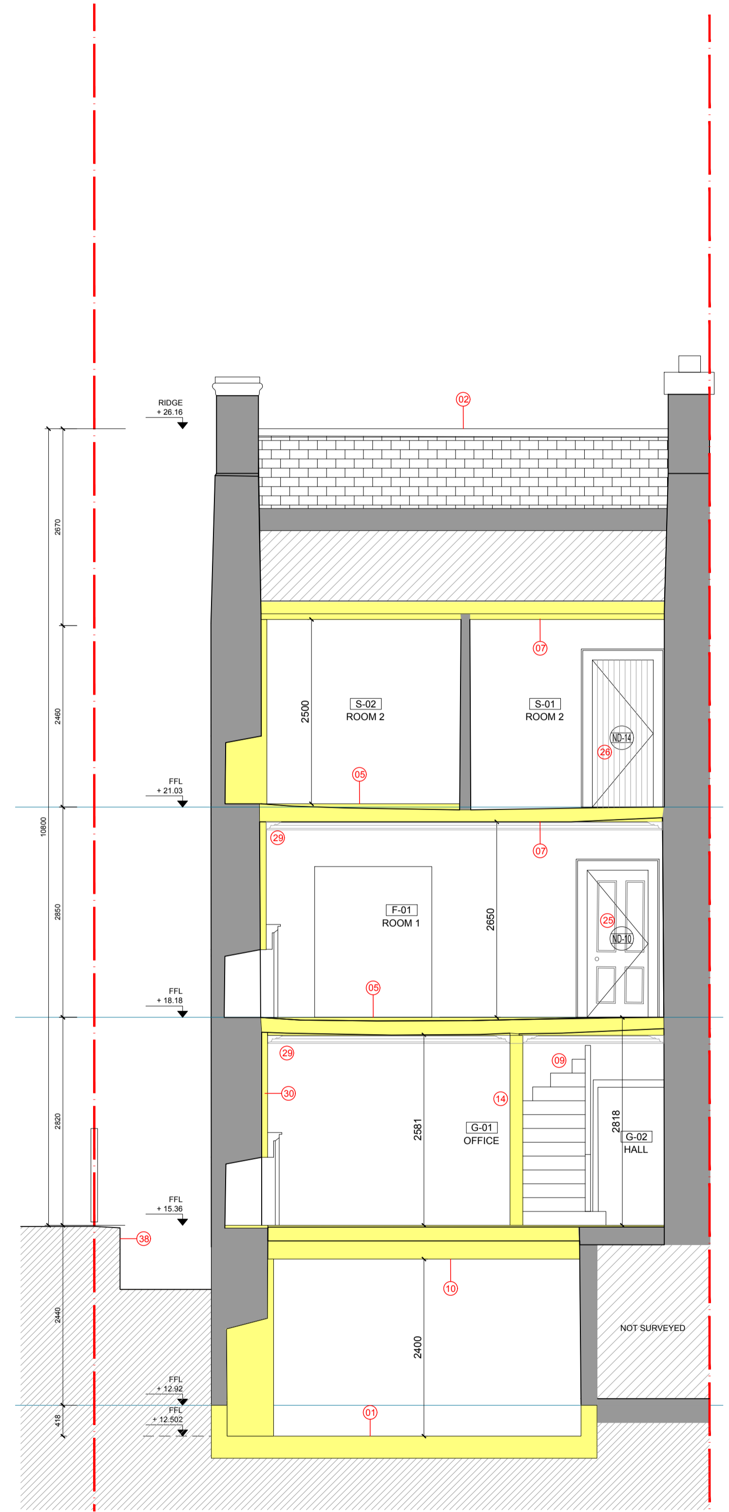
02 PROPOSED SECTION BB 1:50
