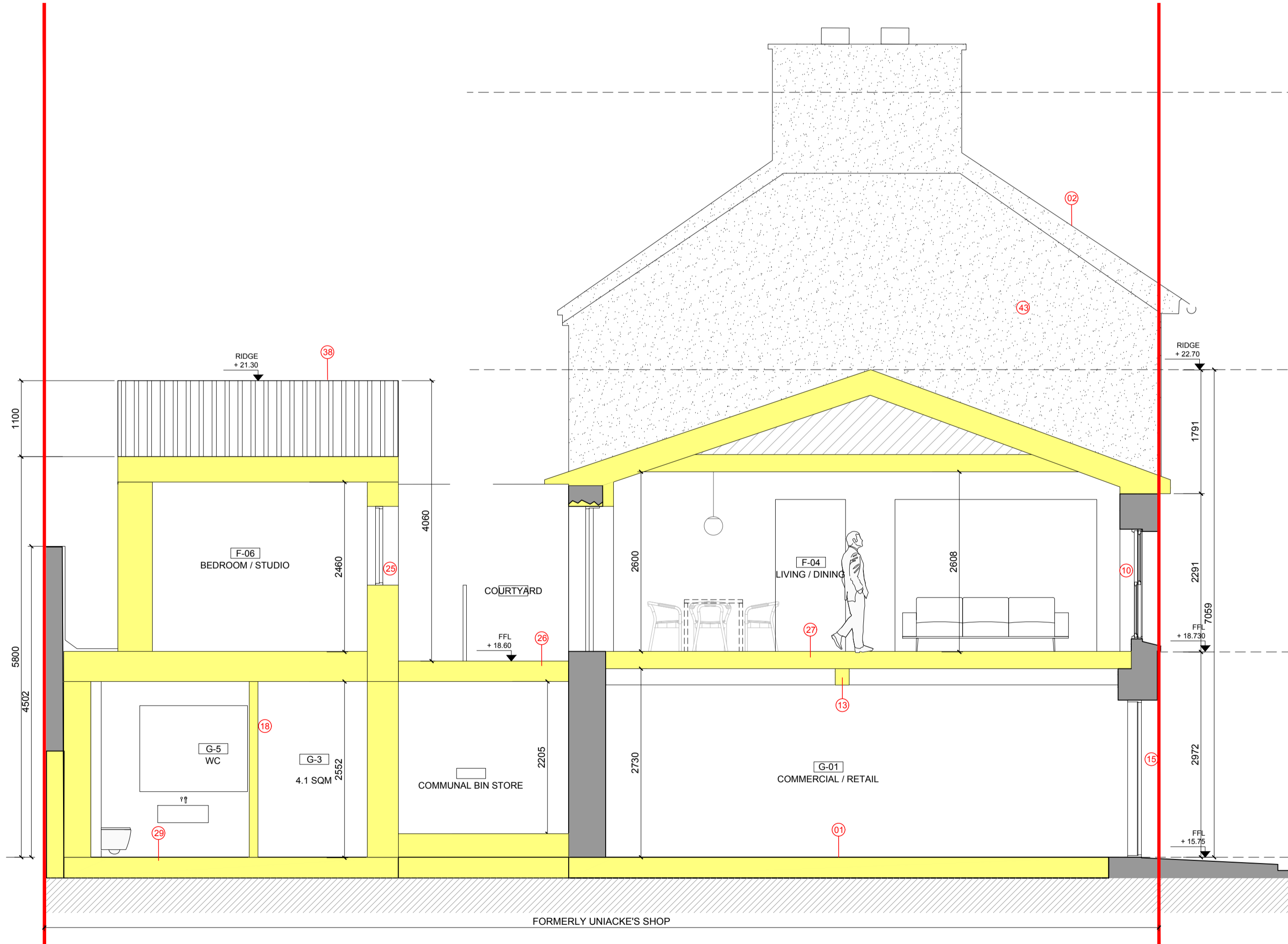
01 PROPOSED SECTION AA 1:50
