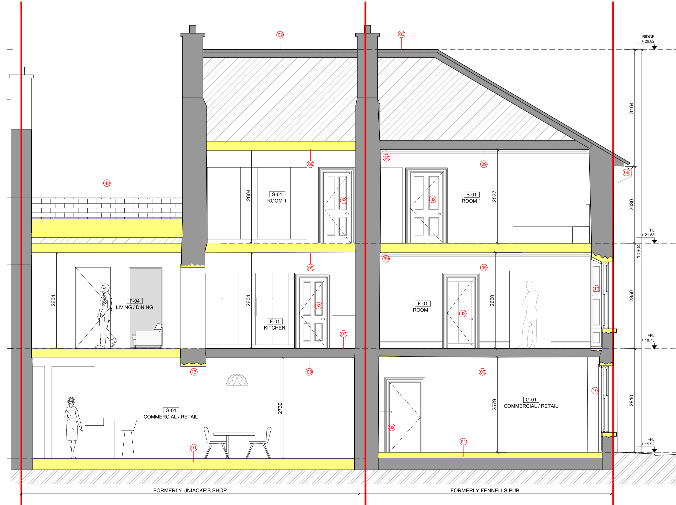
02 PROPOSED SECTION BB 1:50
