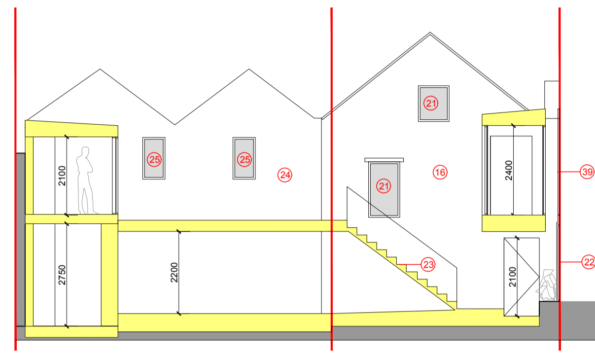
03 PROPOSED SECTION SECTION DIAGRAM CC 1:50
